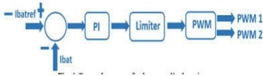
Fig.4 Control system for battery discharging
