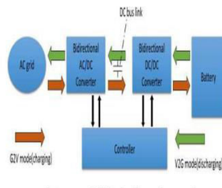
Fig.1 Structure of Bi-directional battery charger topology.
