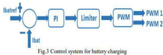
Fig.3 Control system for battery charging
